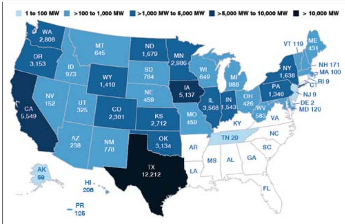
US Wind Power Capacity Installations by State
